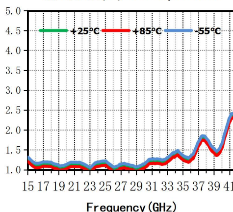
输出驻波(:1) vs. Temperature
