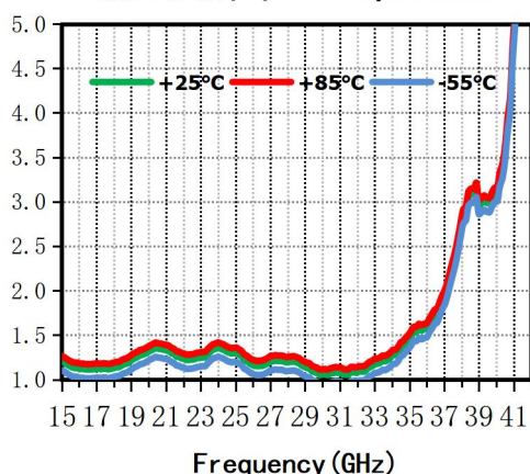
输入驻波(:1) vs. Temperature
