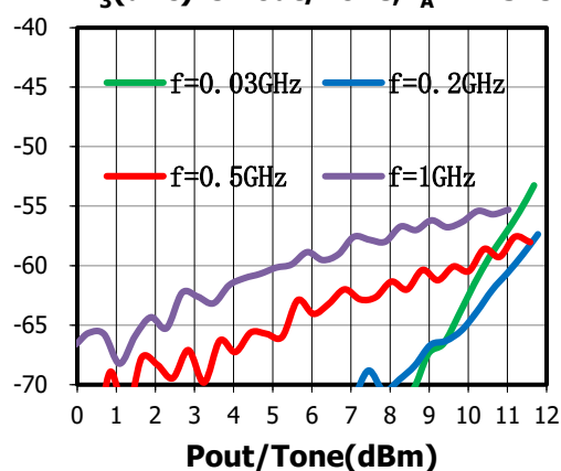
IM_3 (dBc) vs. P_{out}/Tone, T_A = +25^\circ\text{C}
