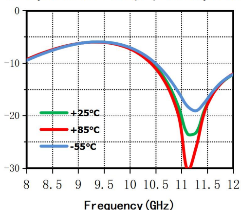
RF Input Return Loss (dB) vs. Temperature
