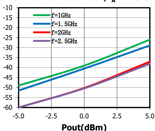
3 RD Harmonic vs. P out , T A = +25°C
