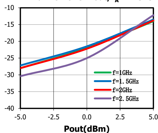
2 ND Harmonic vs. P out , T A = +25°C
