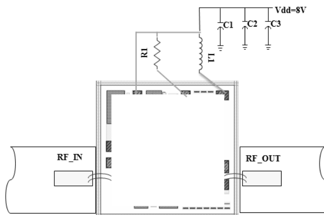
Assembly Diagram
