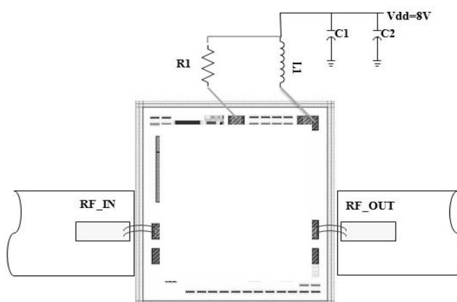
Assembly Diagram
