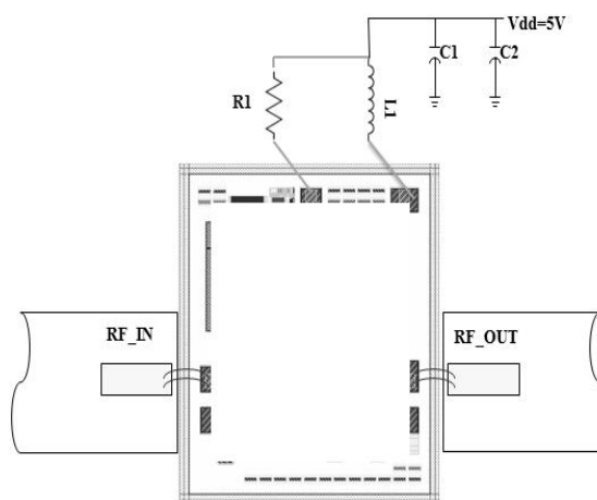
Assembly Diagram
