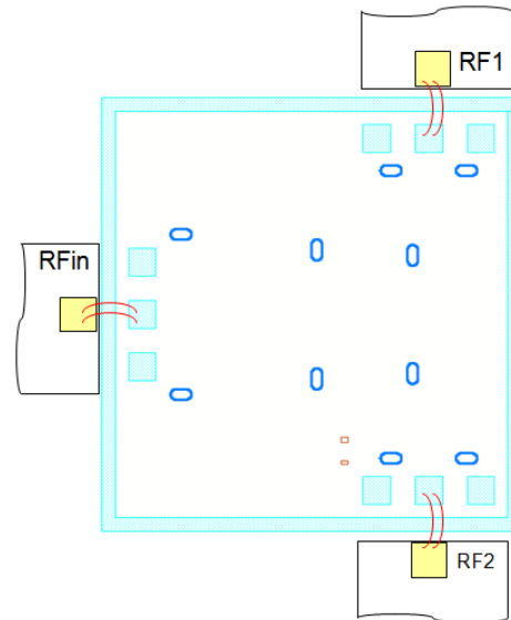
Assembly Diagram
