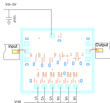
Assembly Diagram
