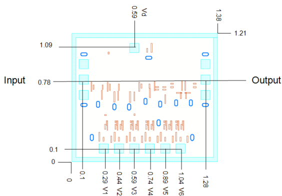
Die Outline (all dimensions in mm)
