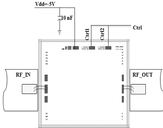
Assembly Diagram
