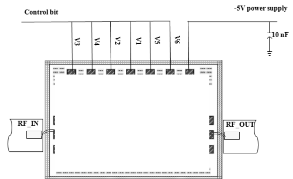
Assembly Diagram
