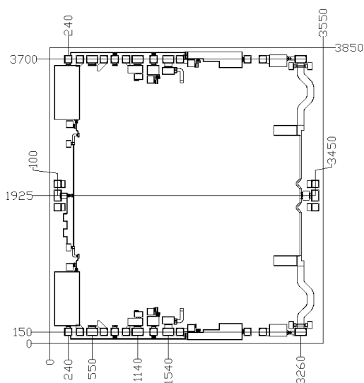
Die Outline (all dimensions in \mu\text{m} )
