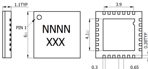
Outline Drawing (all dimensions in mm)
