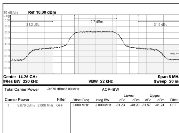
P_{OUT}=36\text{dBm} IDQ=2.45A
