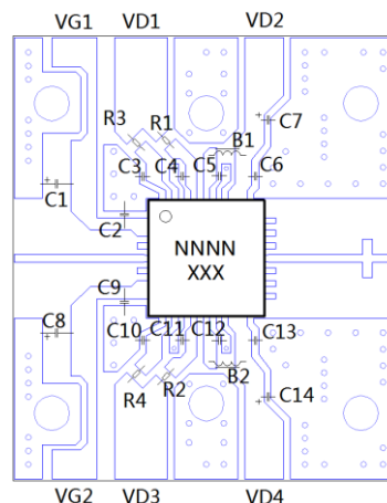
Evaluation PCB Assembly Diagram
