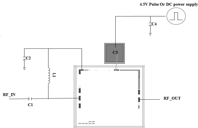
Assembly Diagram
