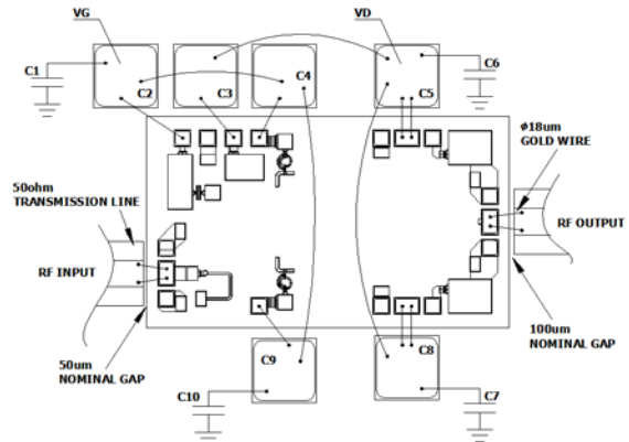
Assembly Diagram
